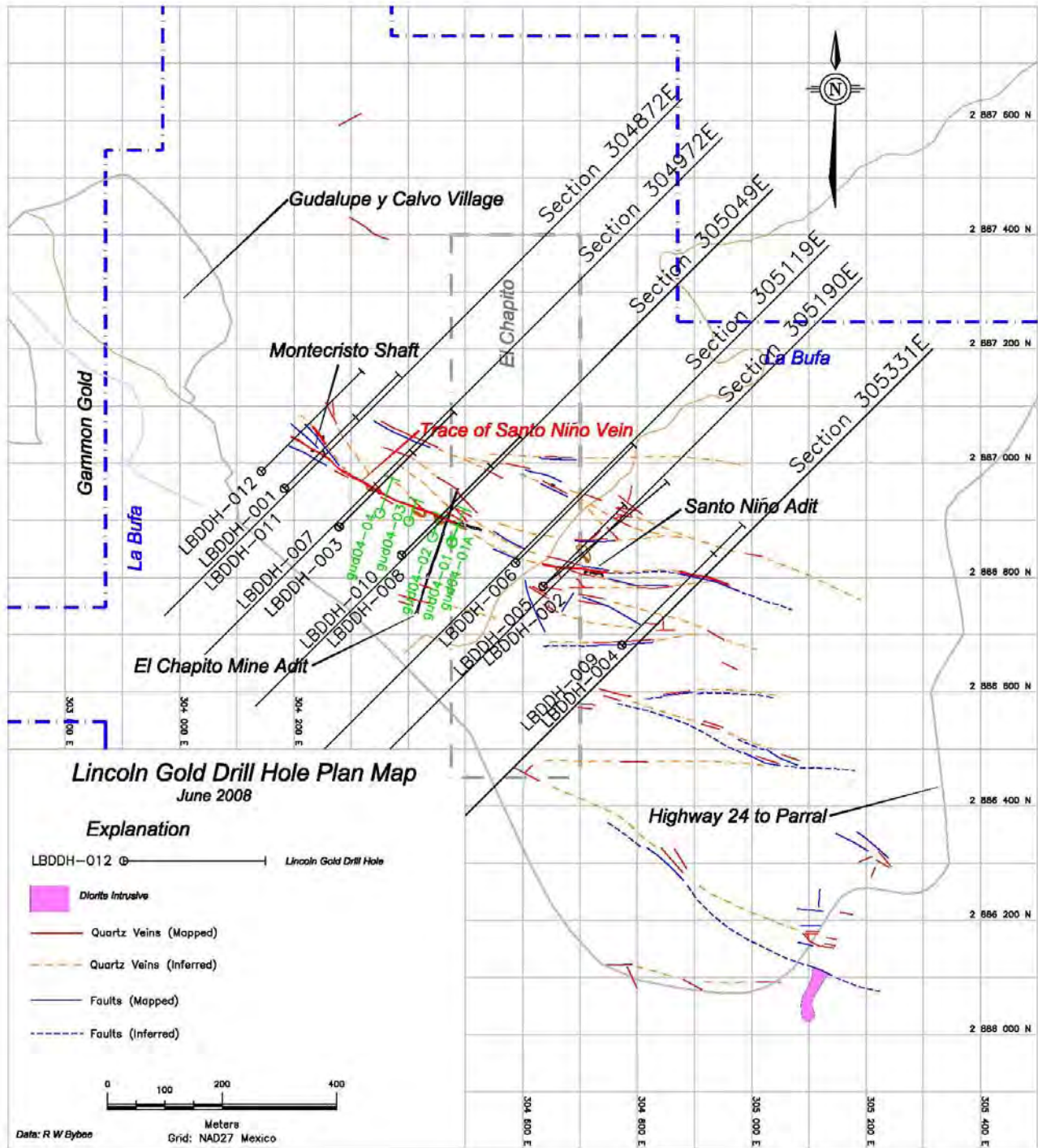
Figure 13.1 Lincoln Gold Drill Hole Plan Map
